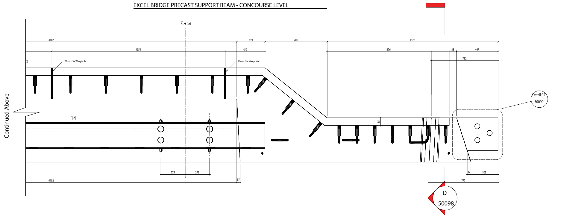
EXCEL BRIDGE PRECAST SUPPORT BEAM - CONCOURSE LEVEL
