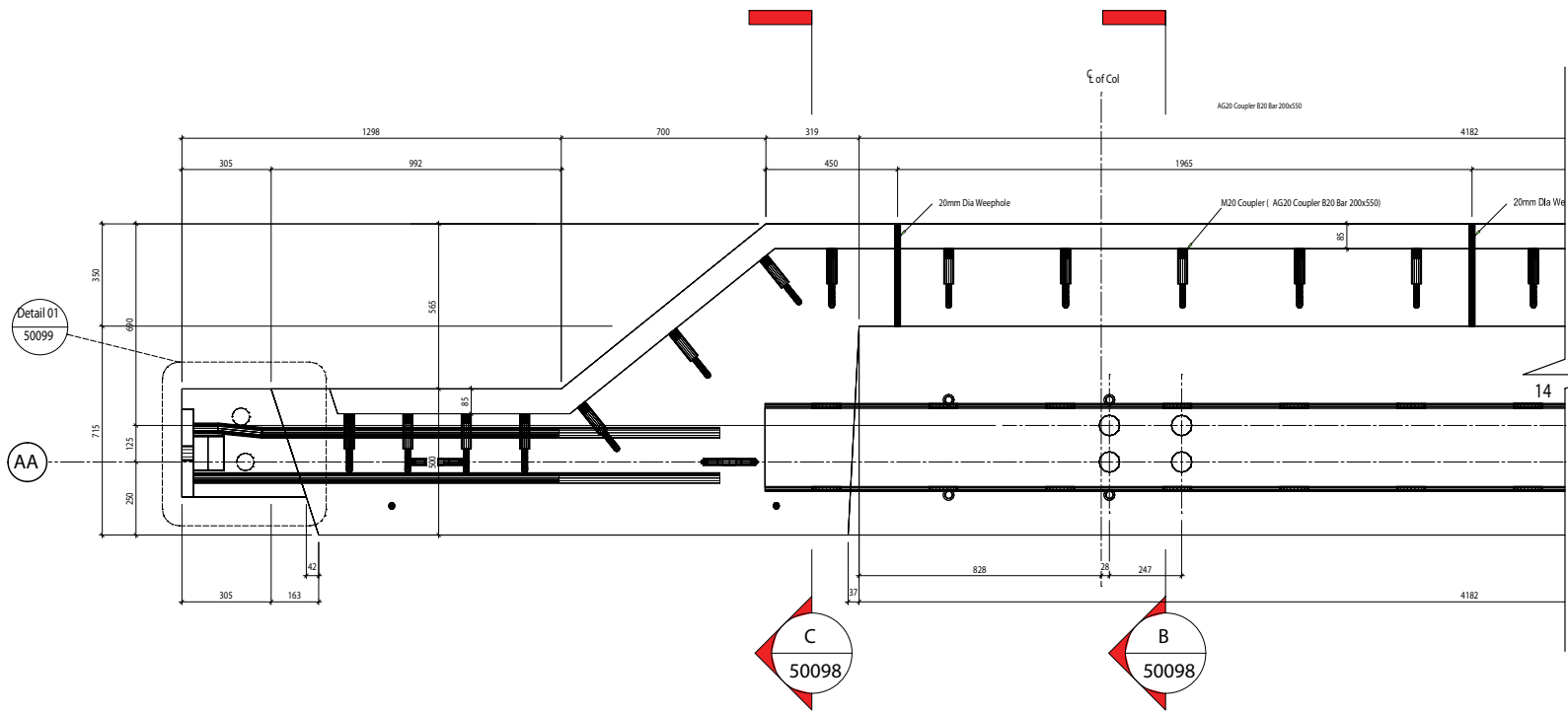
EXCEL BRIDGE PRECAST SUPPORT BEAM - CONCOURSE LEVEL
